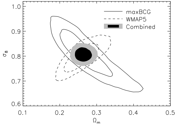
Figure 2 Constraints on the fractional mass density of our universe \Omega_m and the relative variance in the density on 8 Mpc scales \sigma_8 as measured from SDSS data. These results [16] are derived by combining the counts of galaxy clusters with the mass calibrations from gravitational lensing as shown in Figure 1 [12, 13]. The cluster results break degeneracies with other probes such as the cosmic microwave background (WMAP). With DES we will study Dark Energy properties by extending these measurements back in time.
