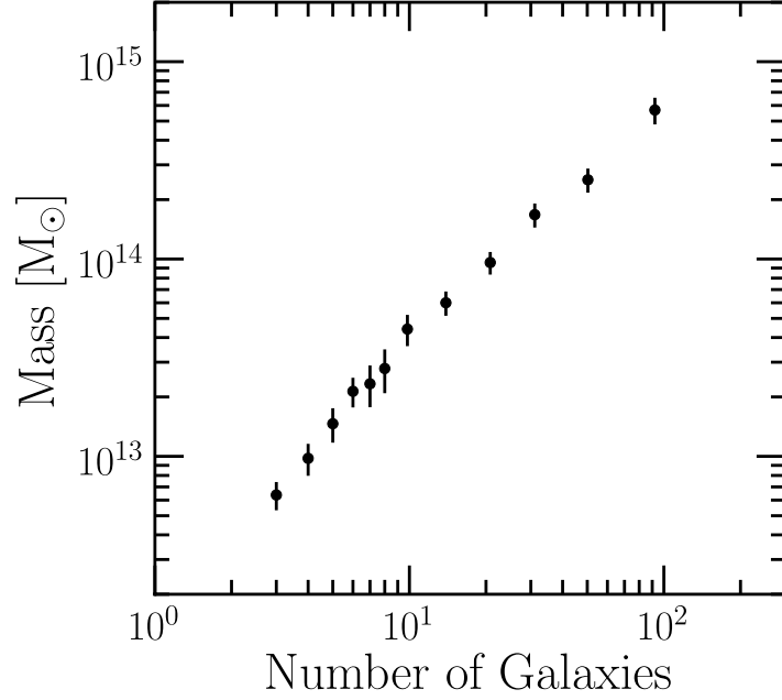
Figure 1 Mean cluster mass as a function of the number of galaxies in the cluster as measured from lensing in SDSS data [12, 13]. This calibration is critical to measuring Dark Energy with galaxy clusters.
