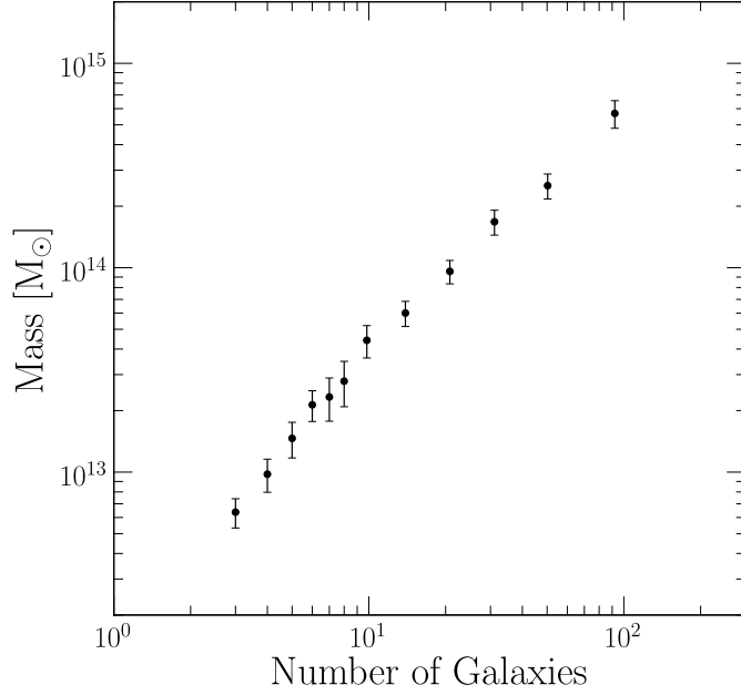
Figure 1 Mean cluster mass as a function of the number of galaxies in the cluster as measured from lensing in SDSS data [12, 13]. This calibration is critical to measuring Dark Energy with galaxy clusters.
