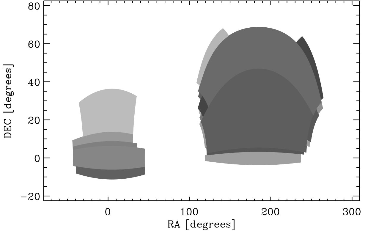
Fig. 1.— BOSS angular window function for the south galactic cap on the left and the north galactic cap on the right. The differently shaded regions represent contiguous rectangular regions in corrected SDSS survey coordinates, used for construction of the window function. Note points with RA > 300^\circ have been wrapped below zero to avoid the 360^\circ crossing point.
