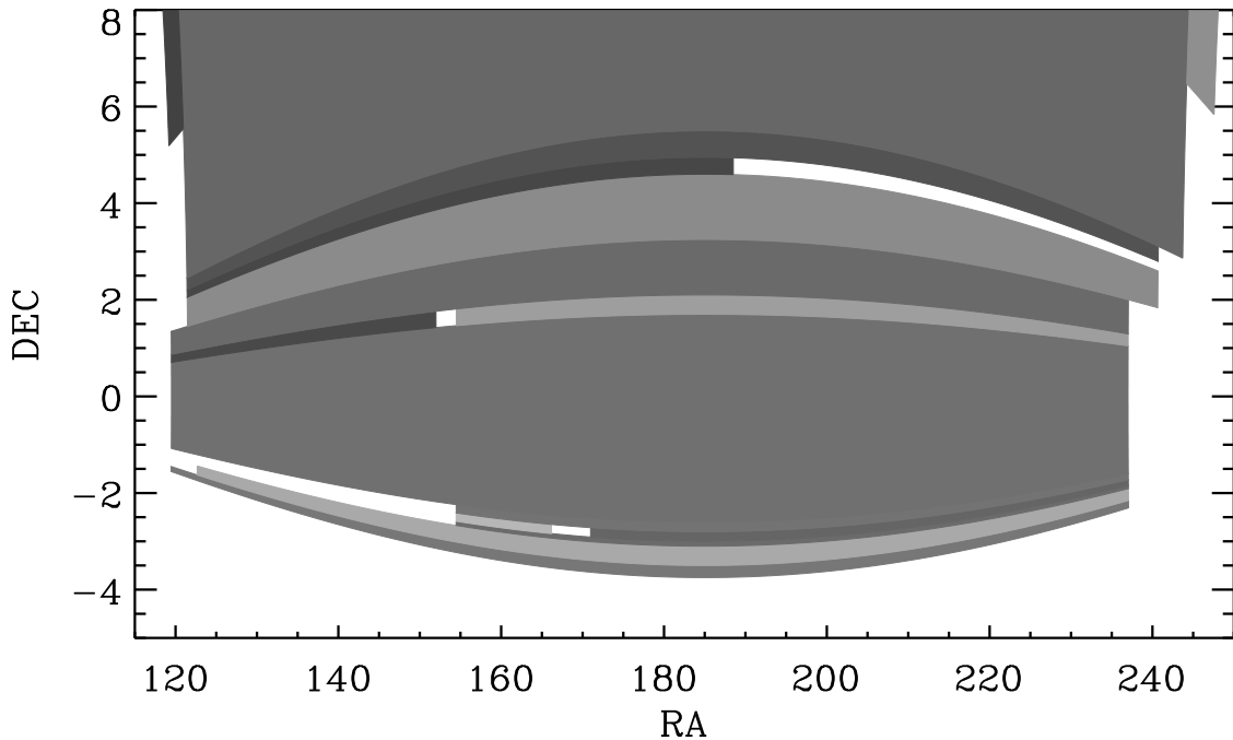
Fig. 2.— A zoomed view of the BOSS footprint, now excluding regions where an amplifier attached to a CCD behind one of the u -band filters was not working. We use this mask during quasar target selection.
